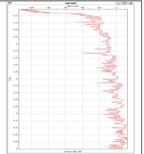
Fig. 12 – Attenuation of amplitude with time line plot after AGC (0.750 s) and t^p ( p = 1.5 ) and 1/\text{rms}
