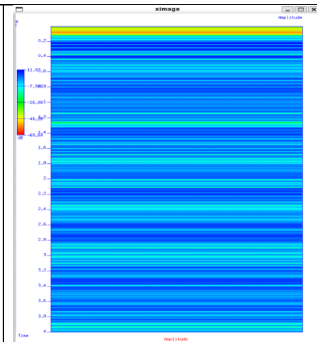
Fig. 5 – Attenuation of amplitude with time colormap diagram after AGC (0.750 s)
