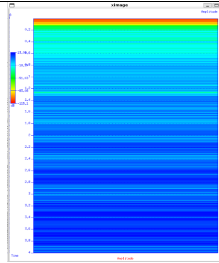
Fig. 11 – Attenuation of amplitude with time colormap diagram after AGC (0.750 s), t^p ( p = 1.5 ) and 1/\text{rms}
