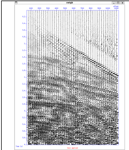
Fig. 10 – Wiggle Plot of seismic Data after AGC(0.750 s), t^p ( p = 1.5 ) and 1/\text{rms}
