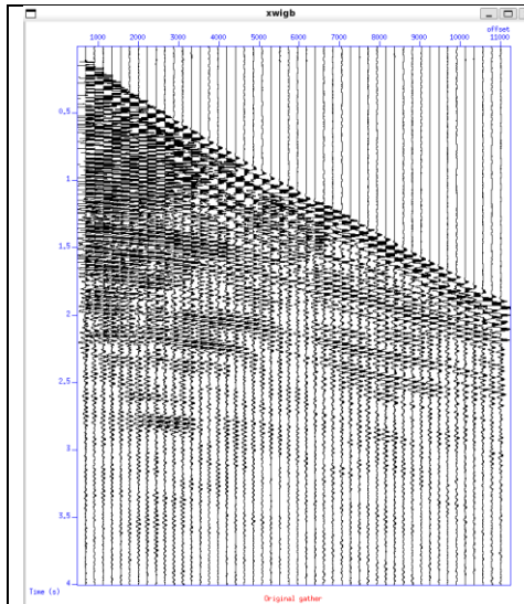
Fig. 1 – Wiggle Plot of seismic Data
